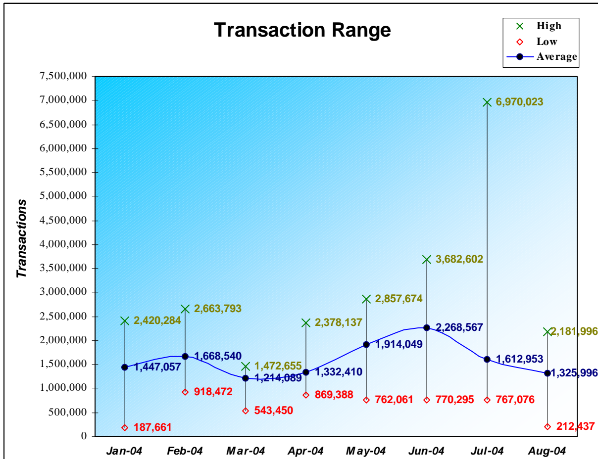
Figure 12: Daily Transaction Range
